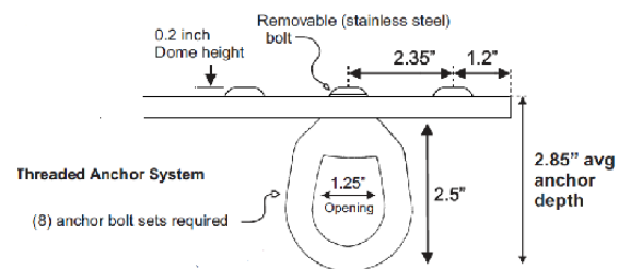
Threaded Anchor System
